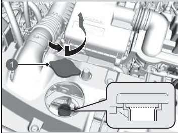
① Kühlerdeckel
